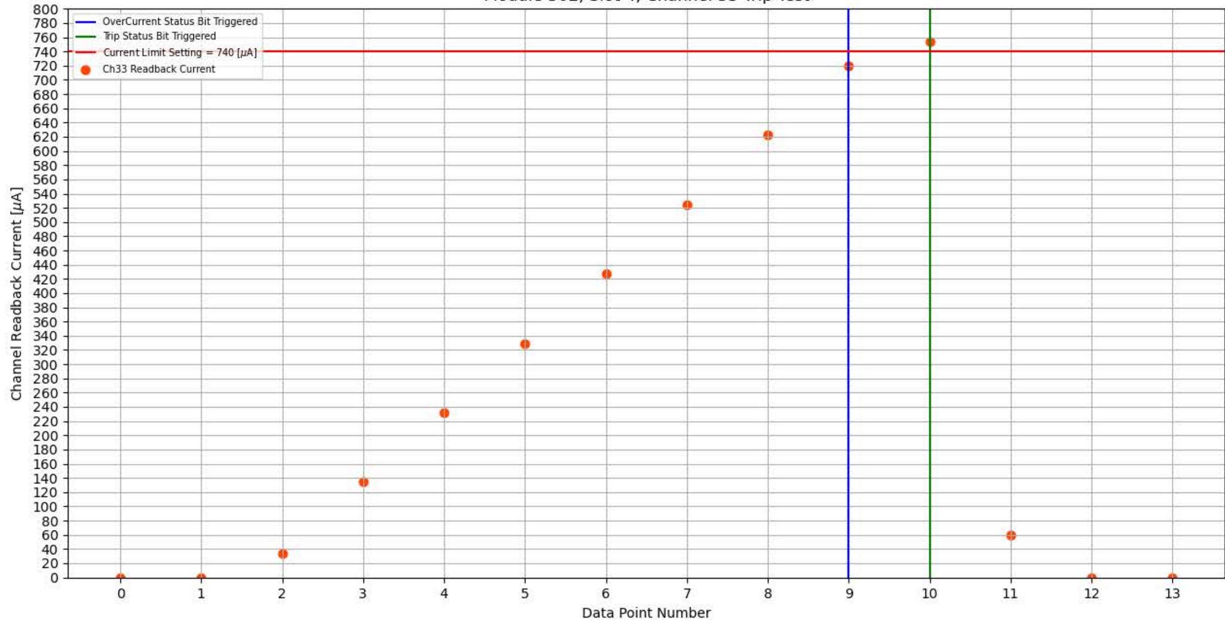
Module 302, Slot 4, Channel 33 Trip Test
