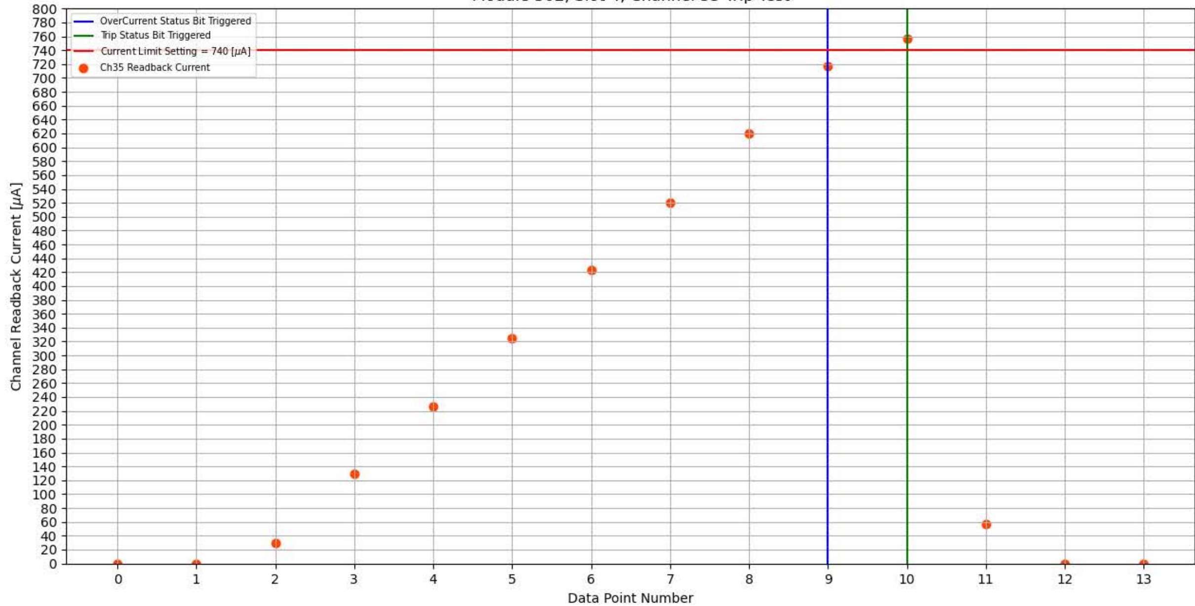
Module 302, Slot 4, Channel 35 Trip Test
