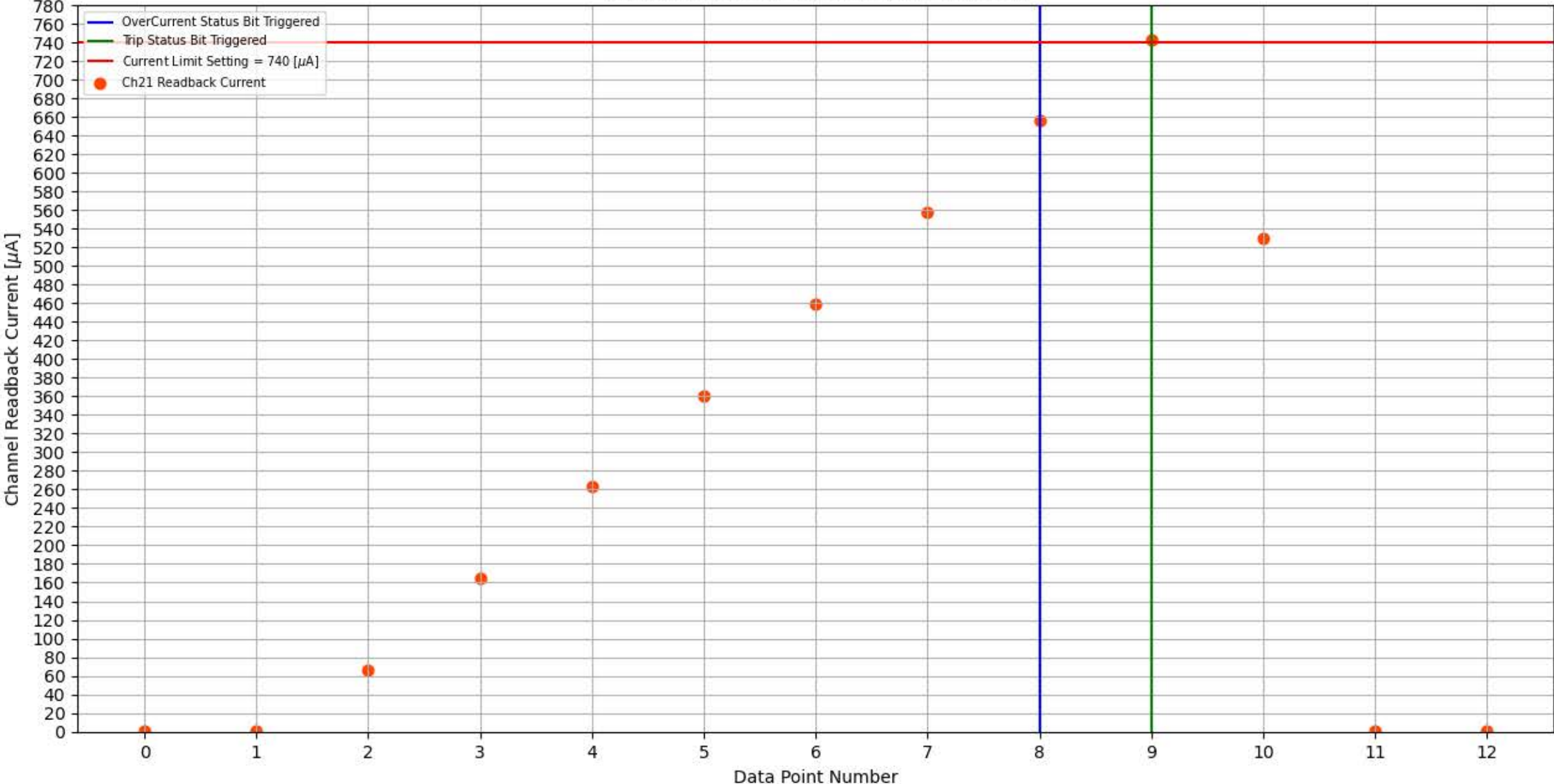
Module 302, Slot 4, Channel 21 Trip Test
