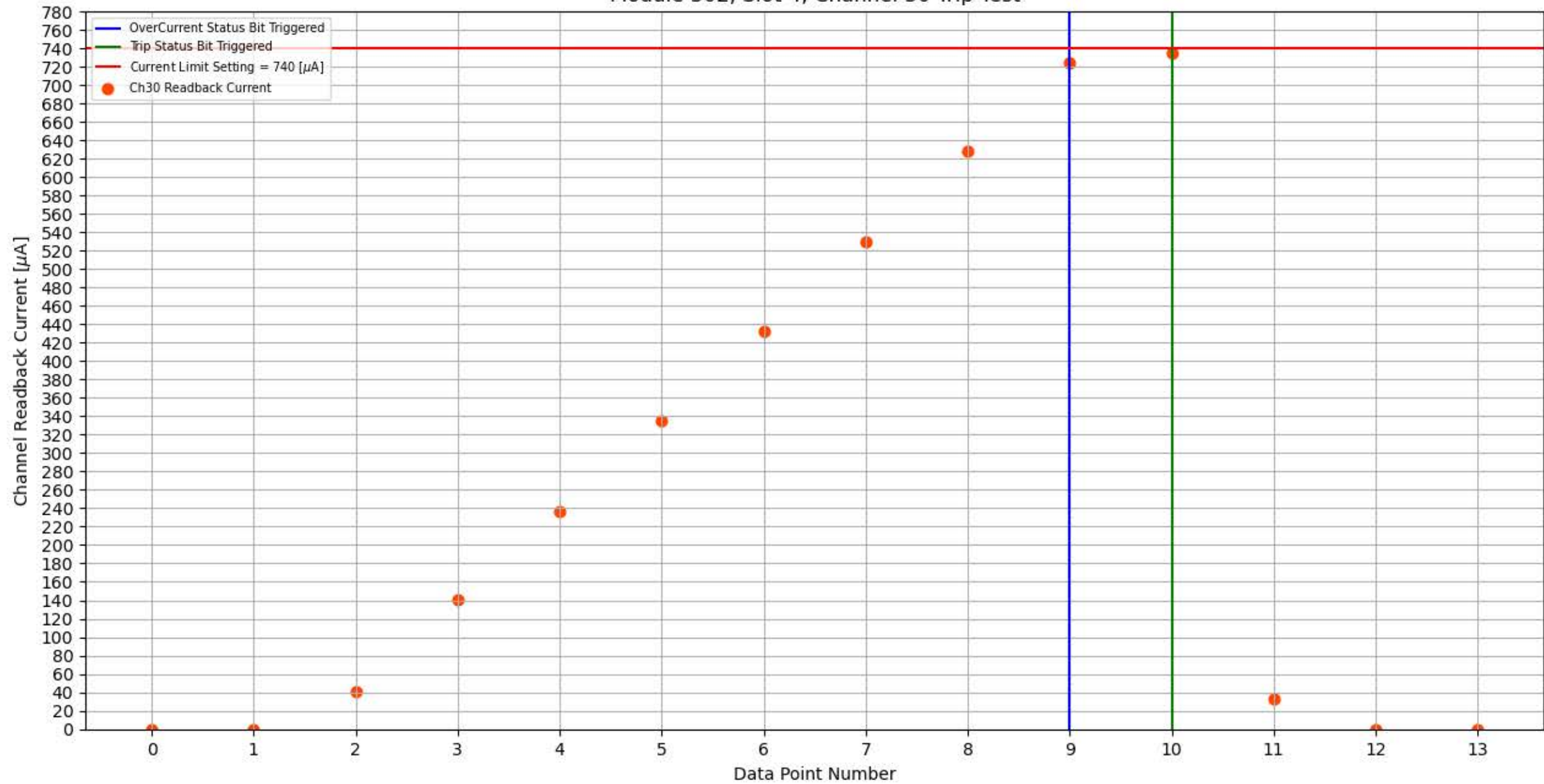
Module 302, Slot 4, Channel 30 Trip Test
