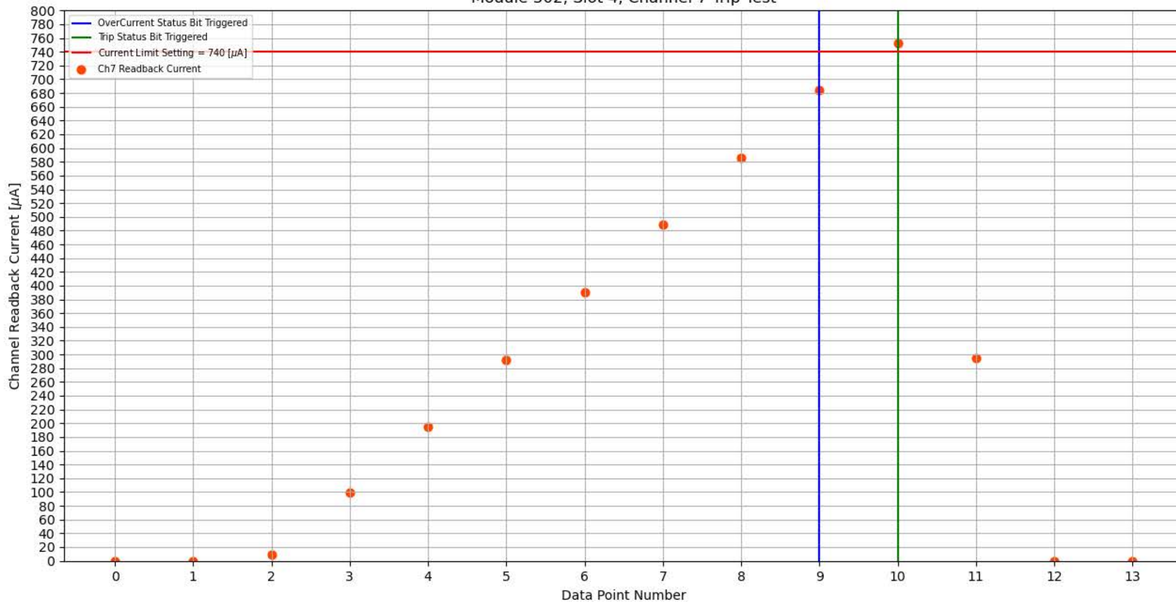
Module 302, Slot 4, Channel 7 Trip Test
