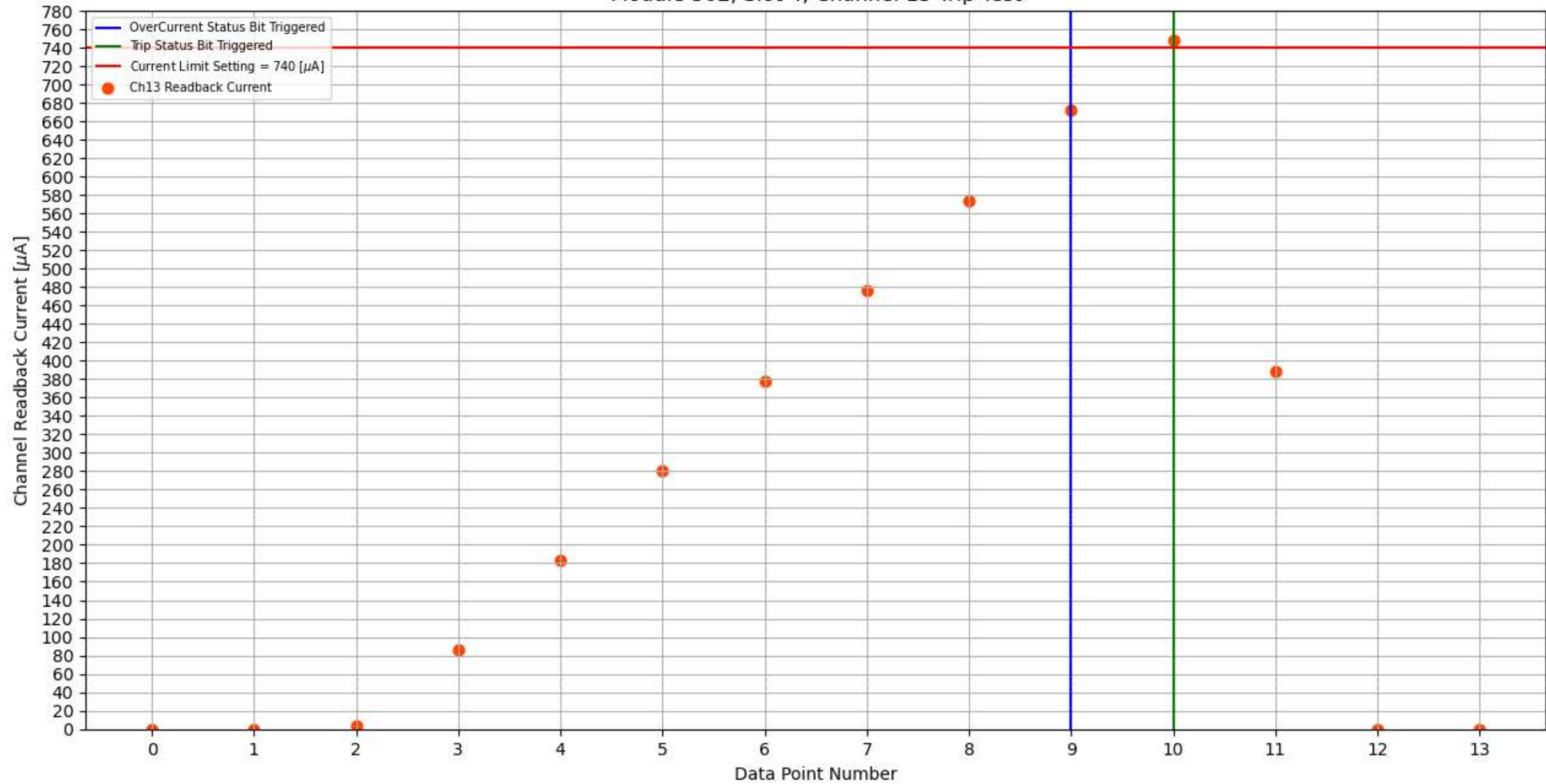
Module 302, Slot 4, Channel 13 Trip Test
