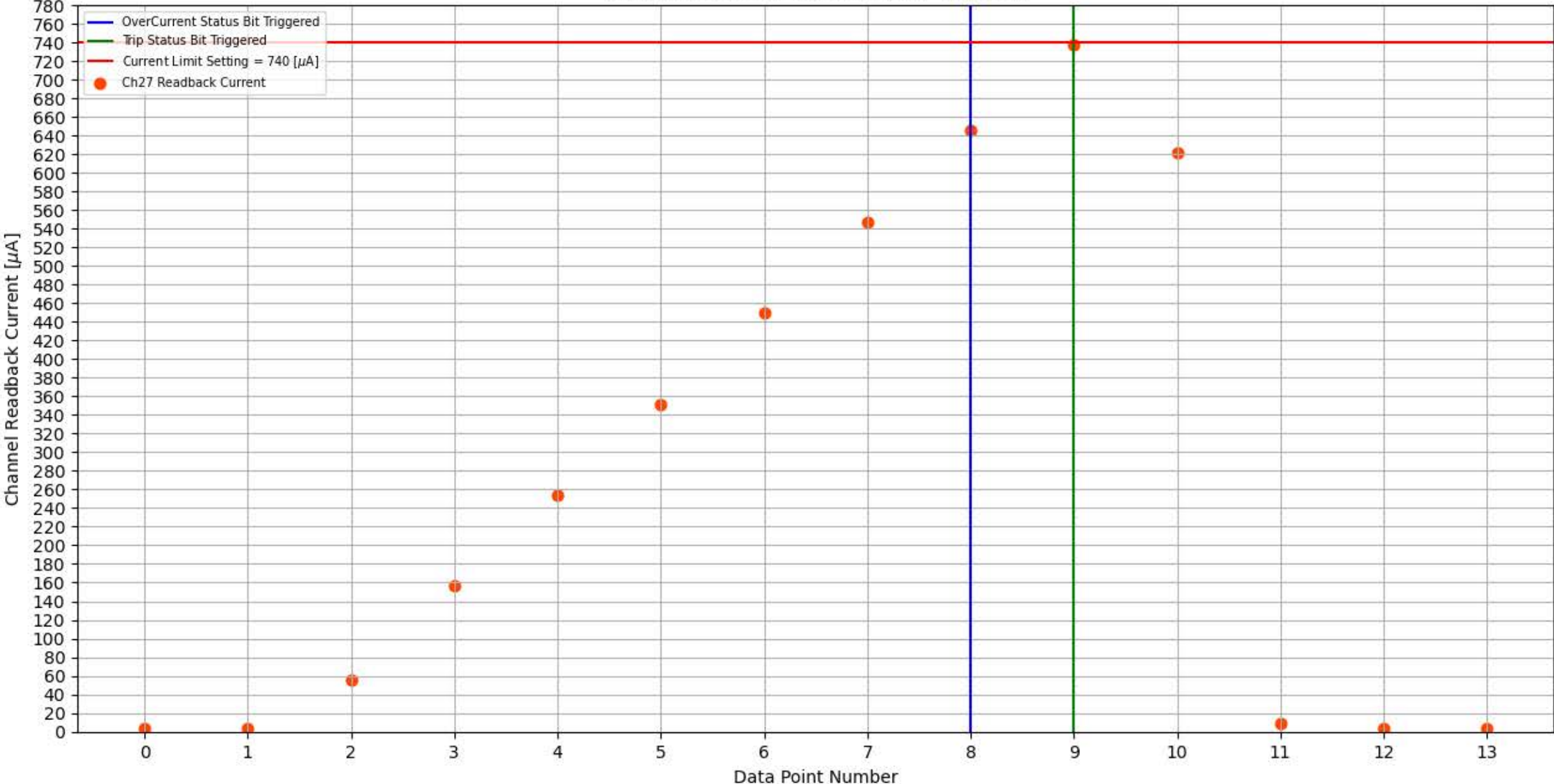
Module 302, Slot 4, Channel 27 Trip Test
