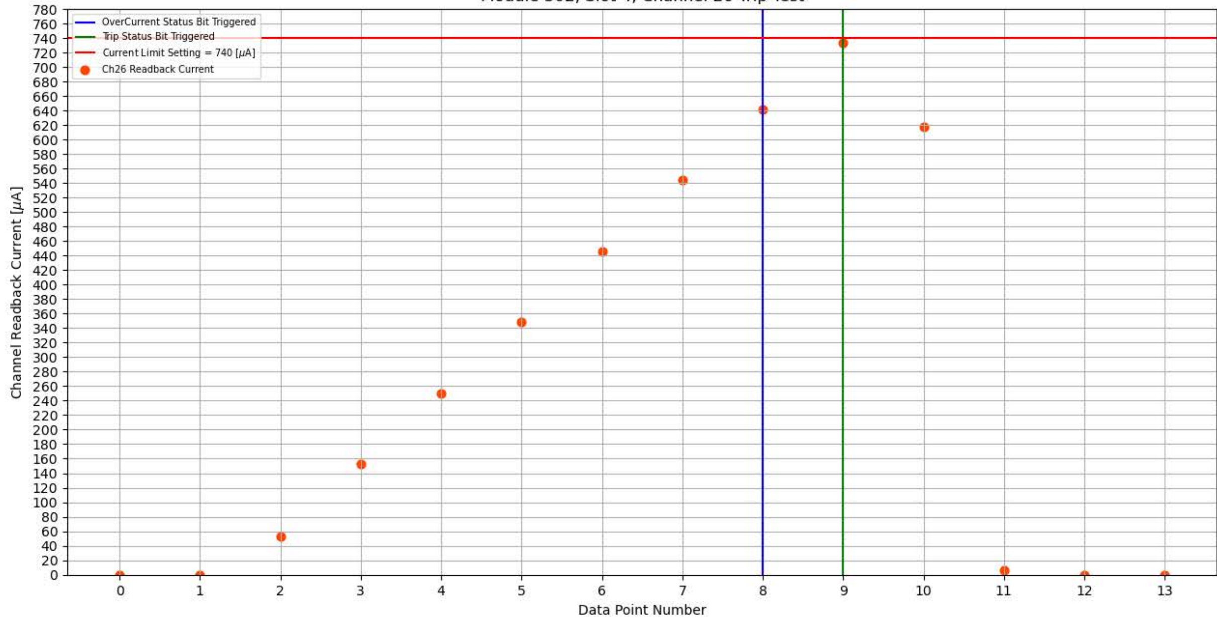
Module 302, Slot 4, Channel 26 Trip Test
