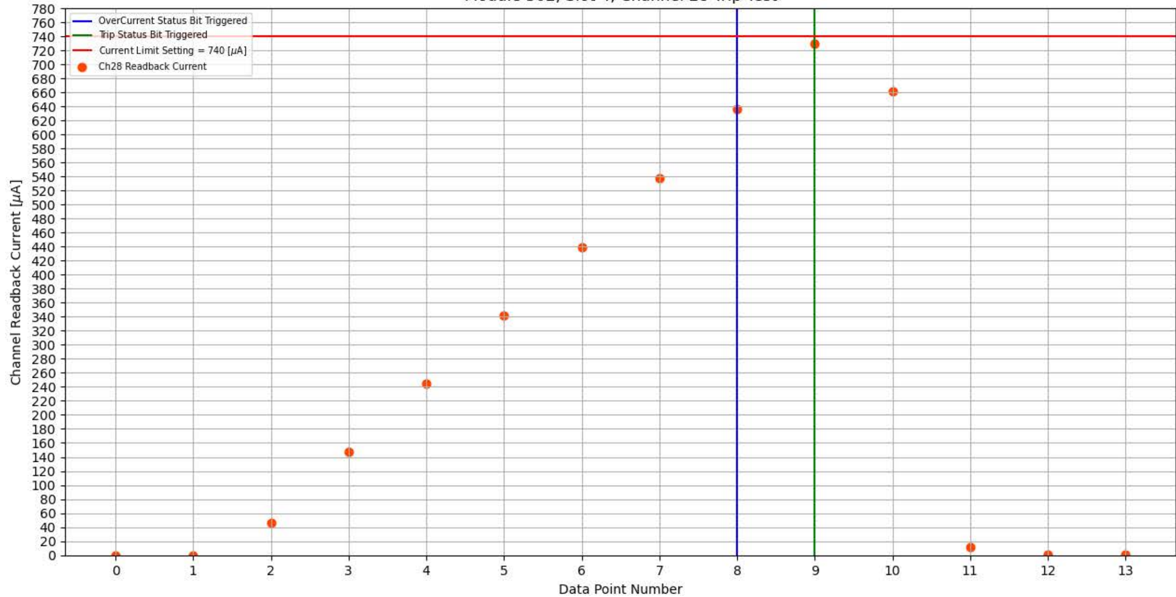
Module 302, Slot 4, Channel 28 Trip Test
