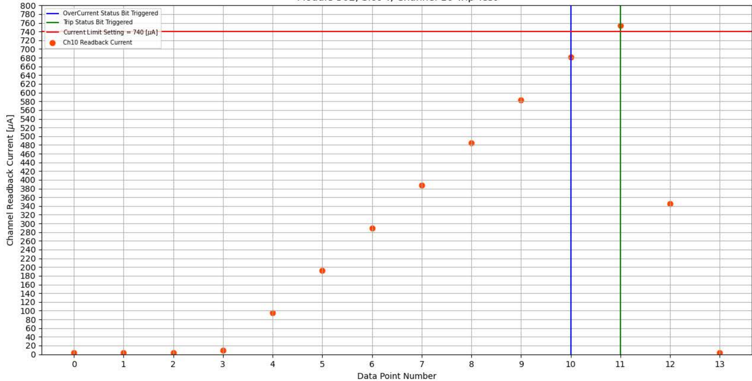
Module 302, Slot 4, Channel 10 Trip Test
