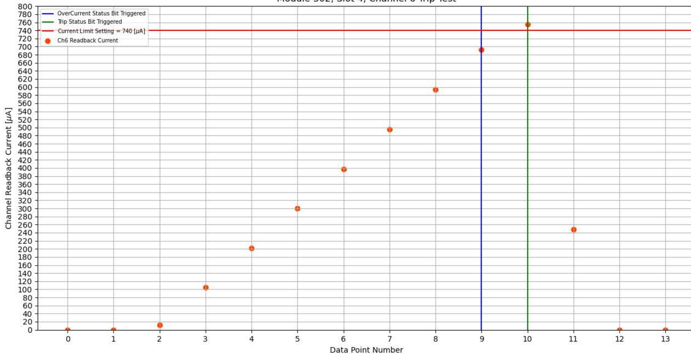
Module 302, Slot 4, Channel 6 Trip Test
