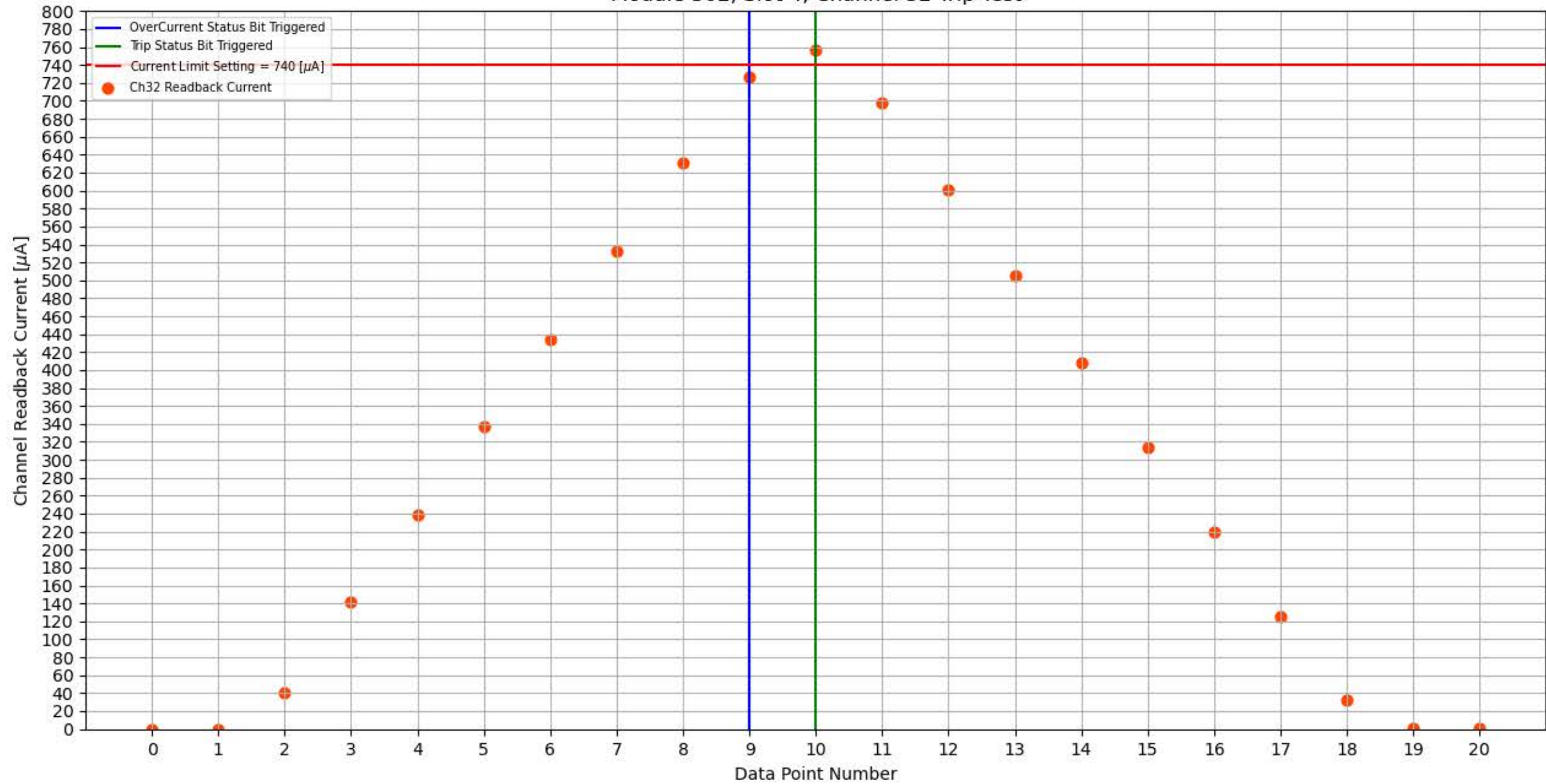
Module 302, Slot 4, Channel 32 Trip Test
