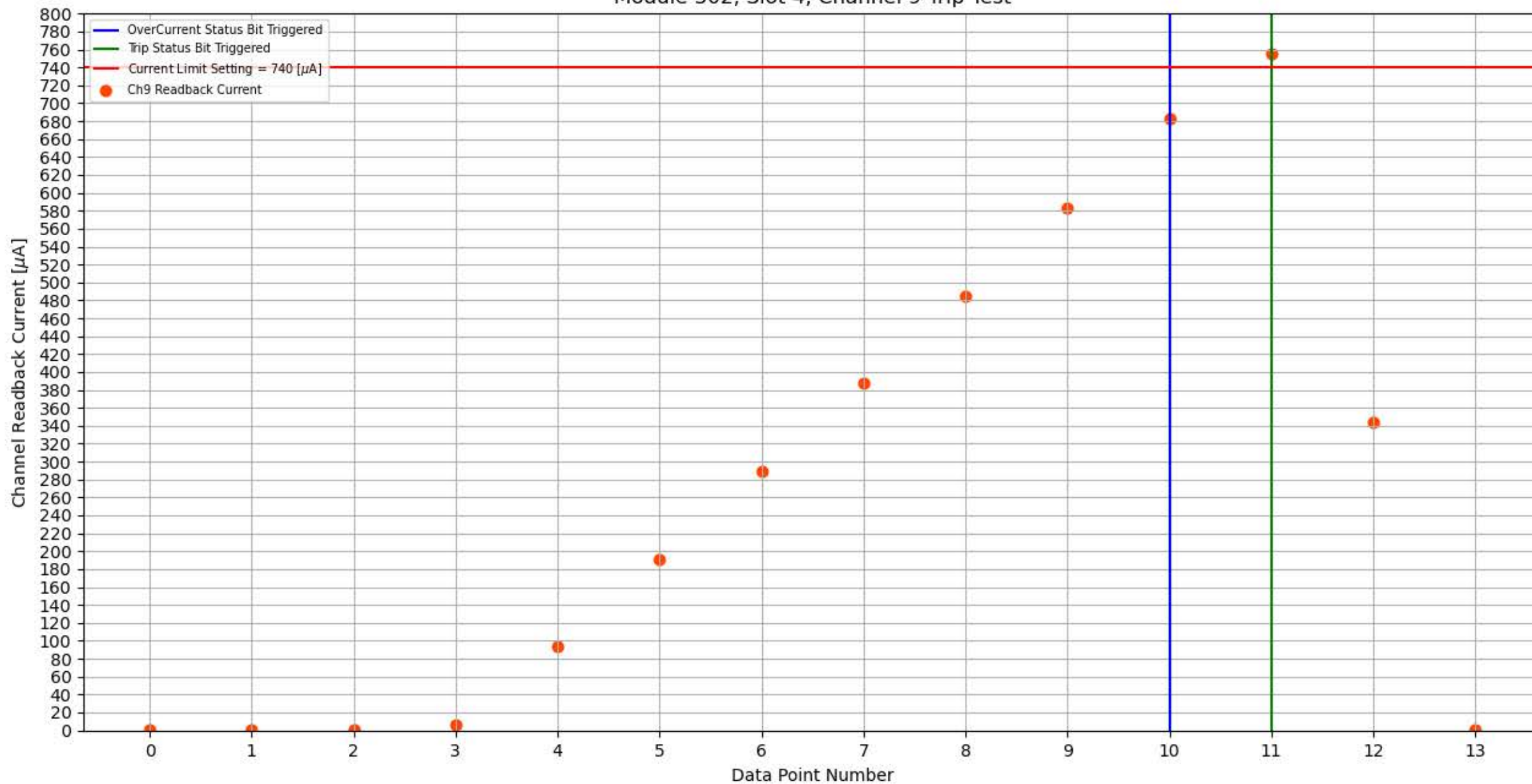
Module 302, Slot 4, Channel 9 Trip Test
