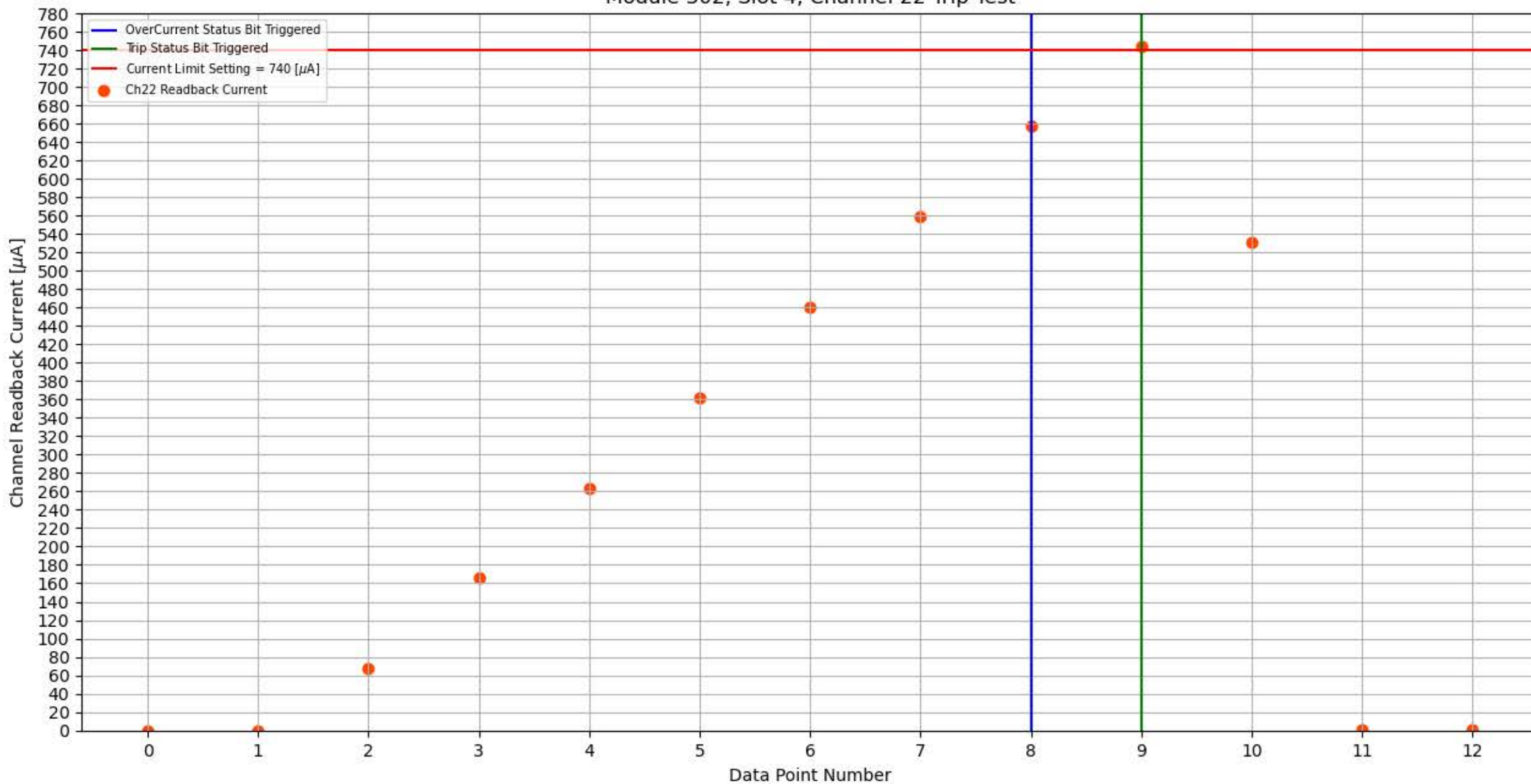
Module 302, Slot 4, Channel 22 Trip Test
