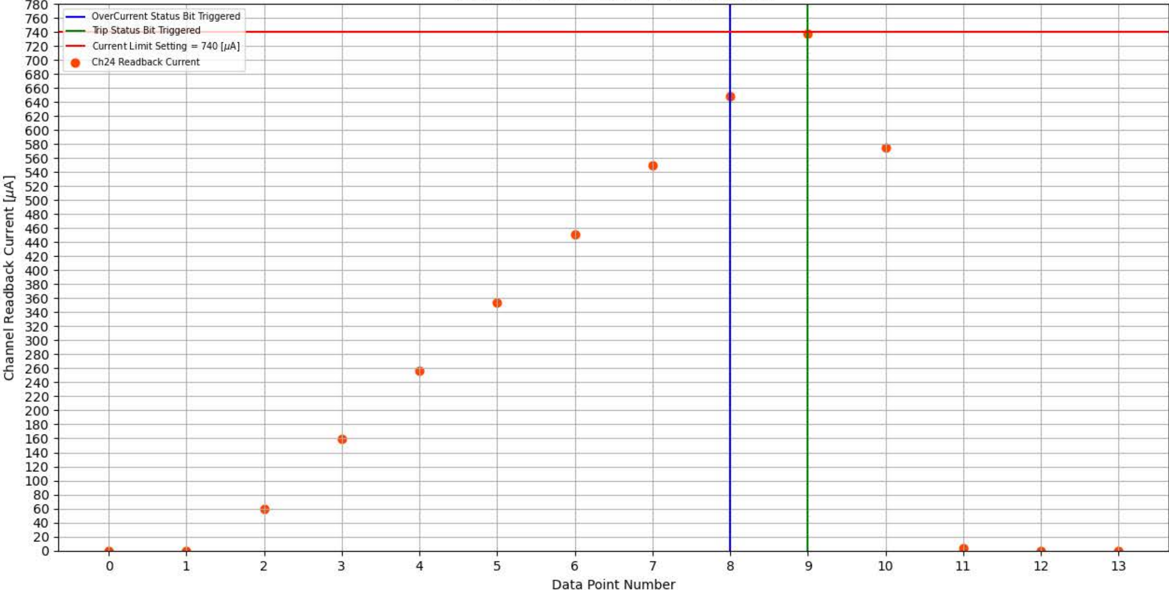
Module 302, Slot 4, Channel 24 Trip Test
