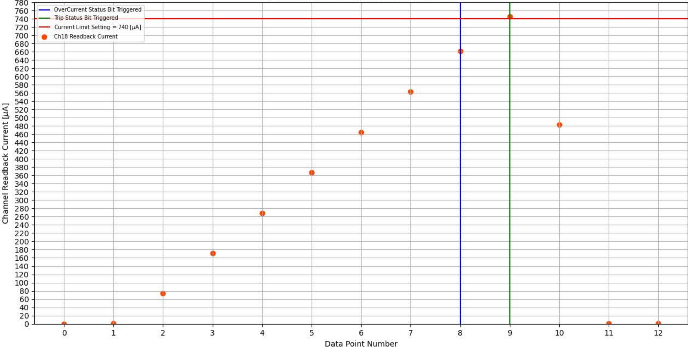
Module 302, Slot 4, Channel 18 Trip Test
