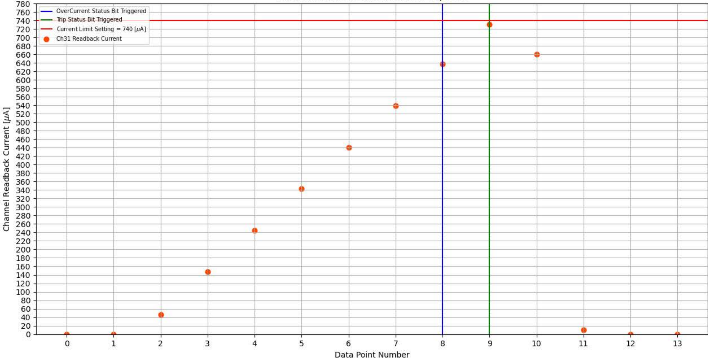
Module 302, Slot 4, Channel 31 Trip Test
