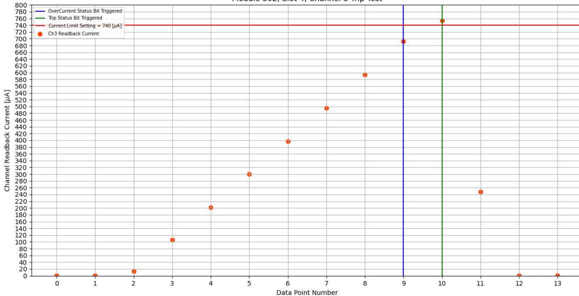
Module 302, Slot 4, Channel 3 Trip Test
