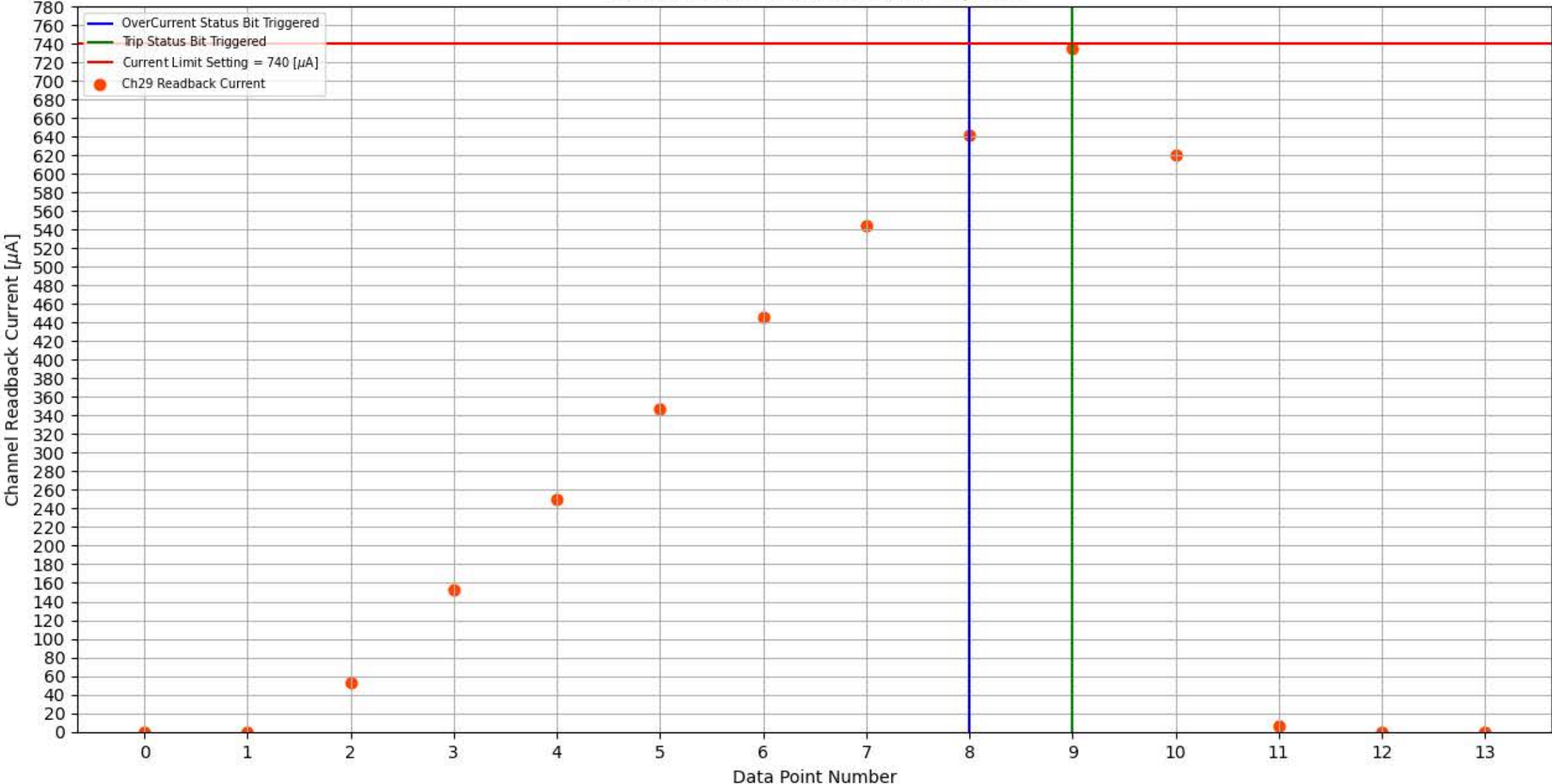
Module 302, Slot 4, Channel 29 Trip Test
