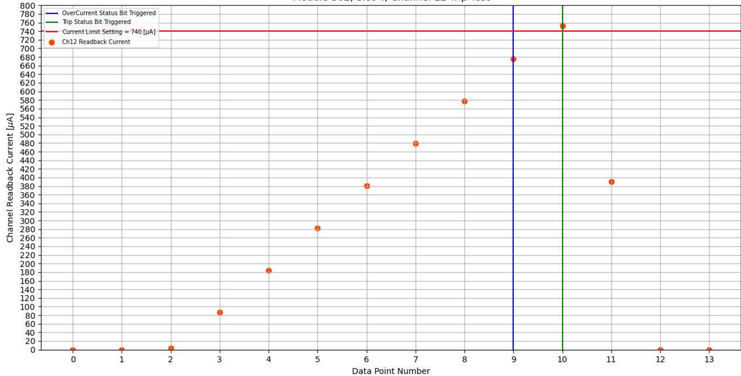
Module 302, Slot 4, Channel 12 Trip Test
