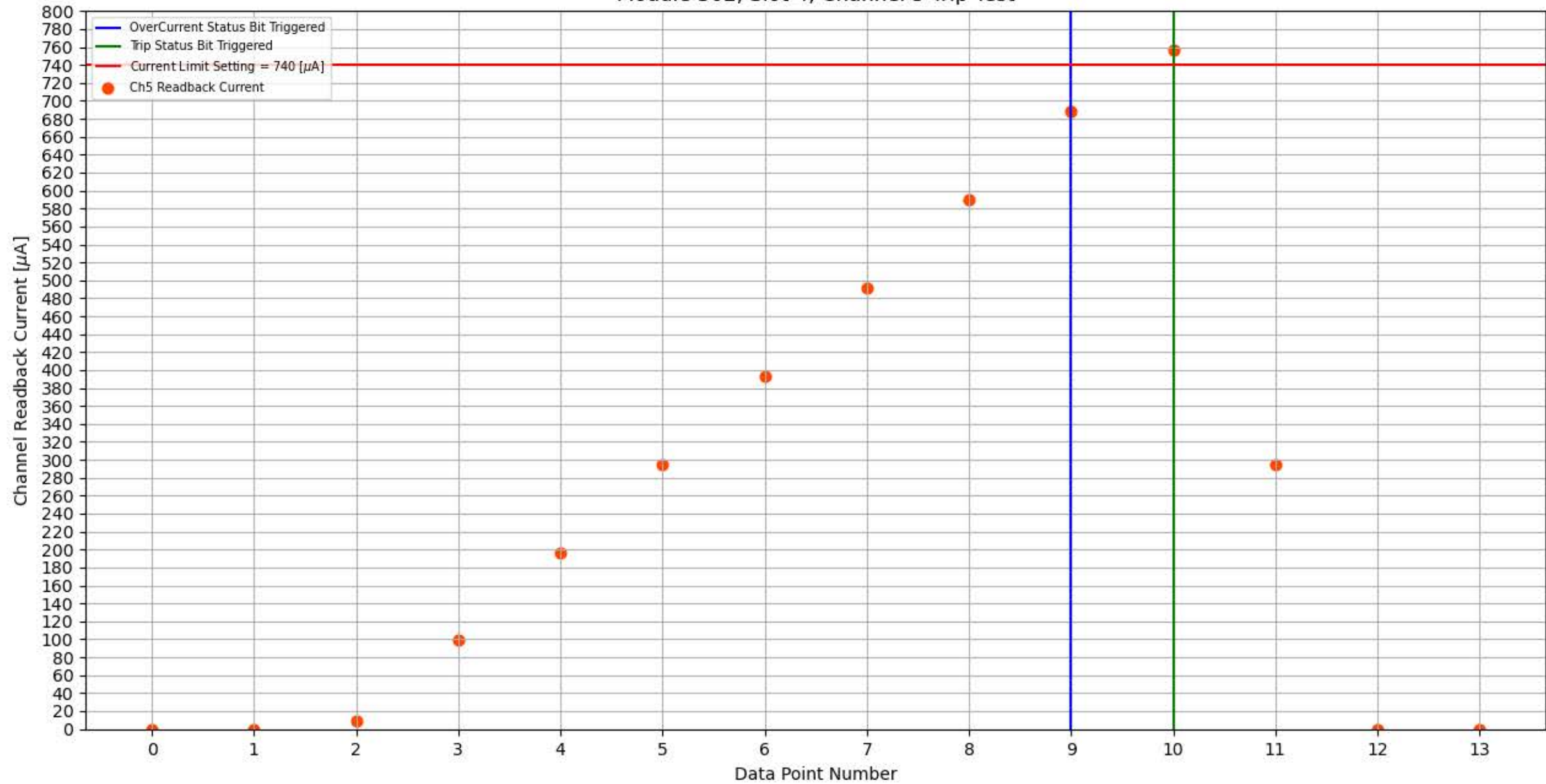
Module 302, Slot 4, Channel 5 Trip Test
