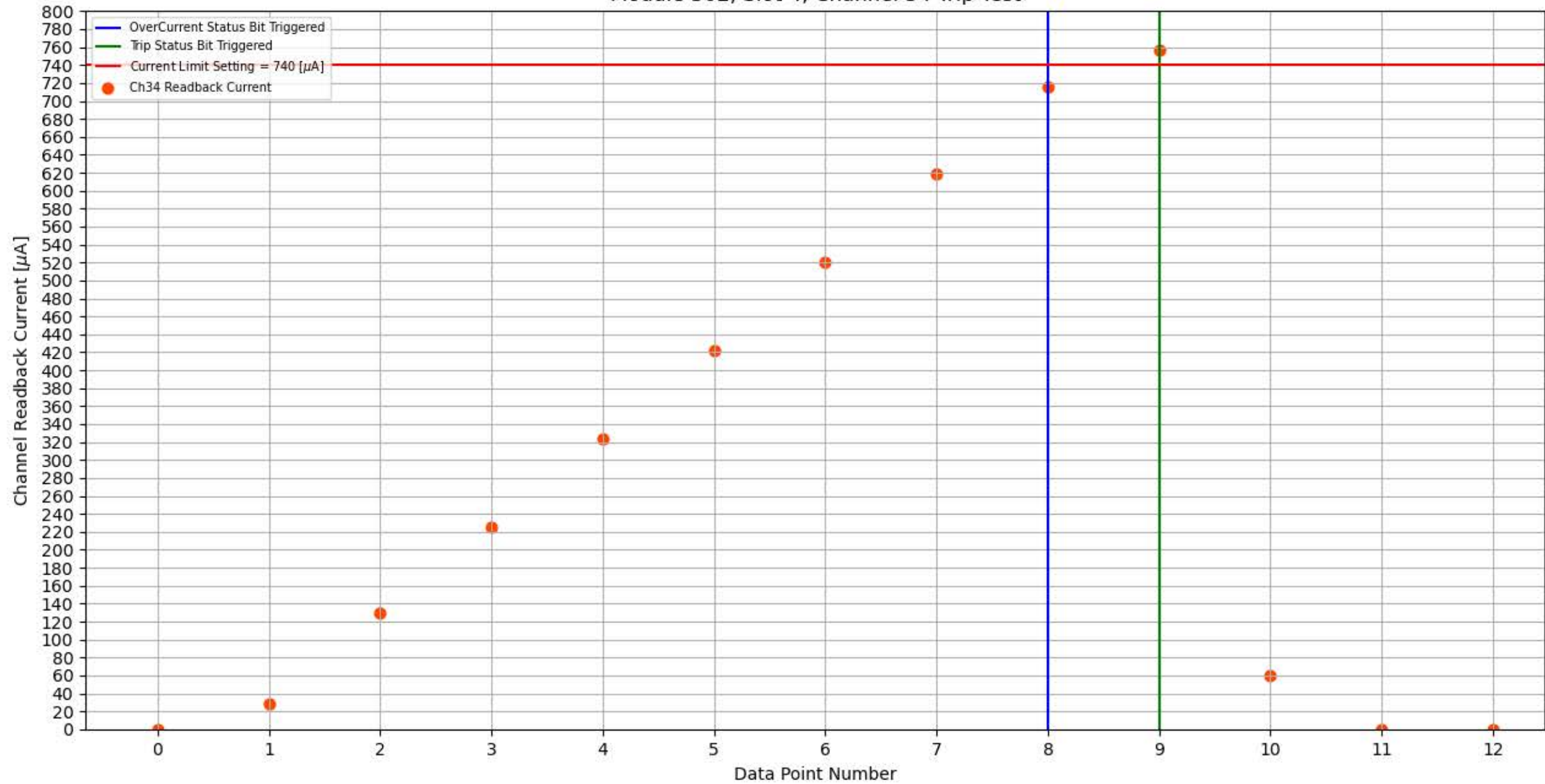
Module 302, Slot 4, Channel 34 Trip Test
