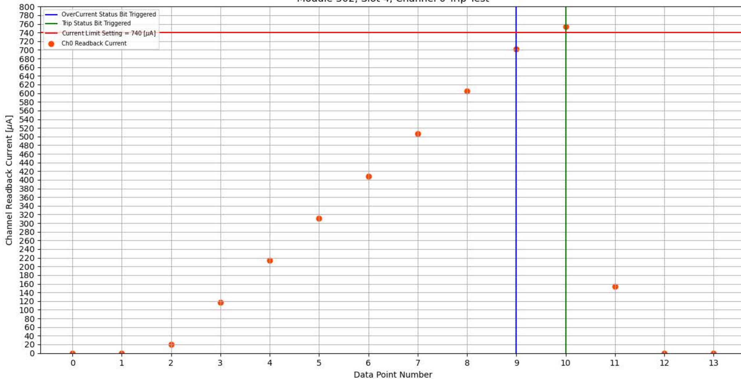
Module 302, Slot 4, Channel 0 Trip Test
