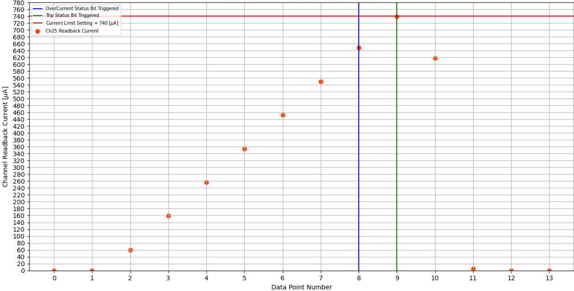
Module 302, Slot 4, Channel 25 Trip Test
