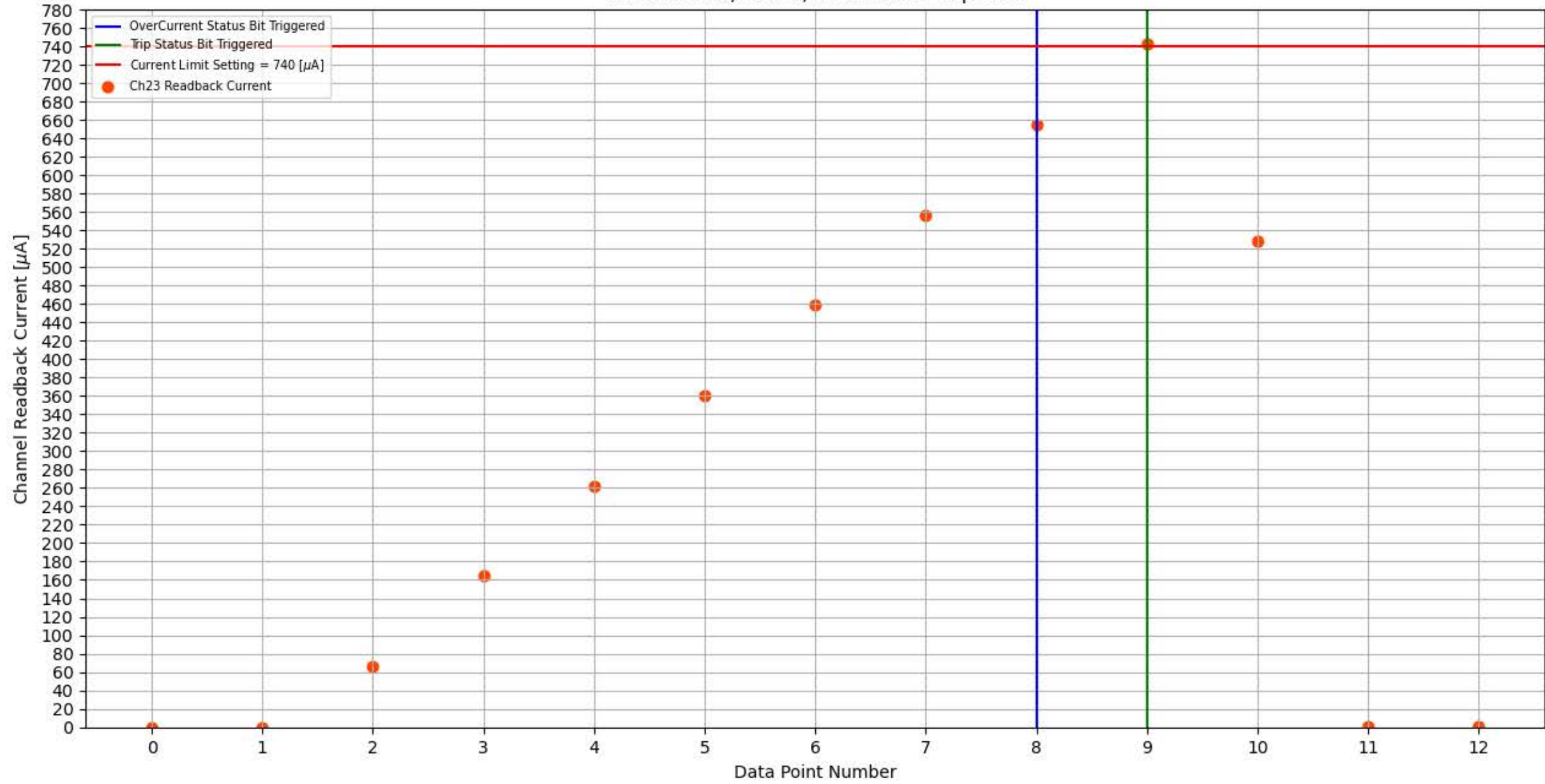
Module 302, Slot 4, Channel 23 Trip Test
