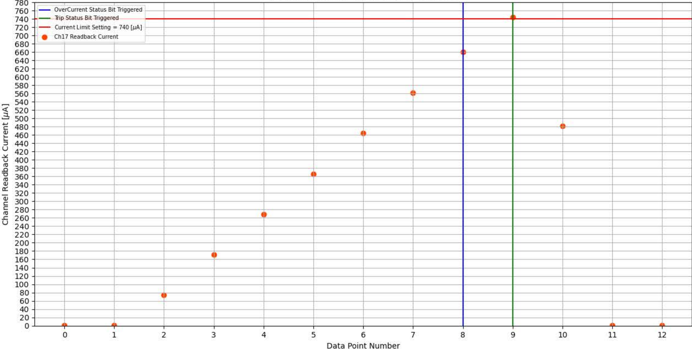
Module 302, Slot 4, Channel 17 Trip Test
