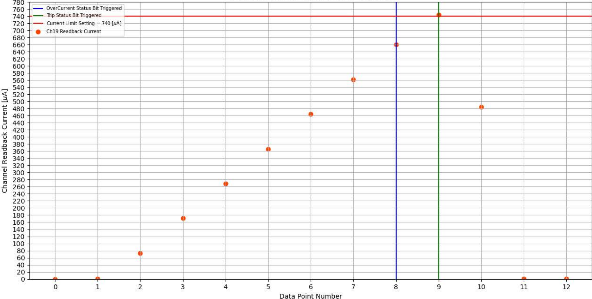
Module 302, Slot 4, Channel 19 Trip Test
