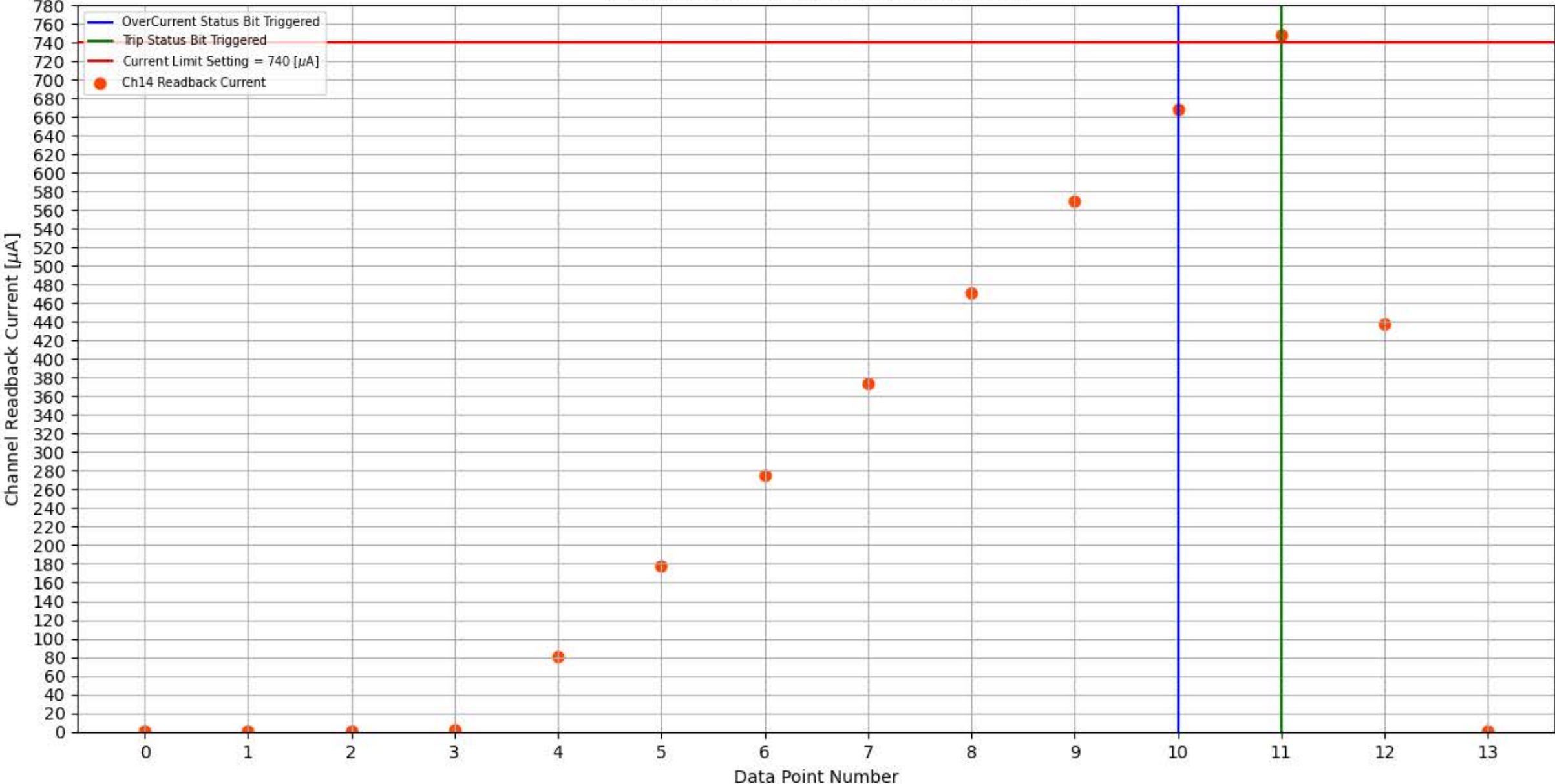
Module 302, Slot 4, Channel 14 Trip Test
