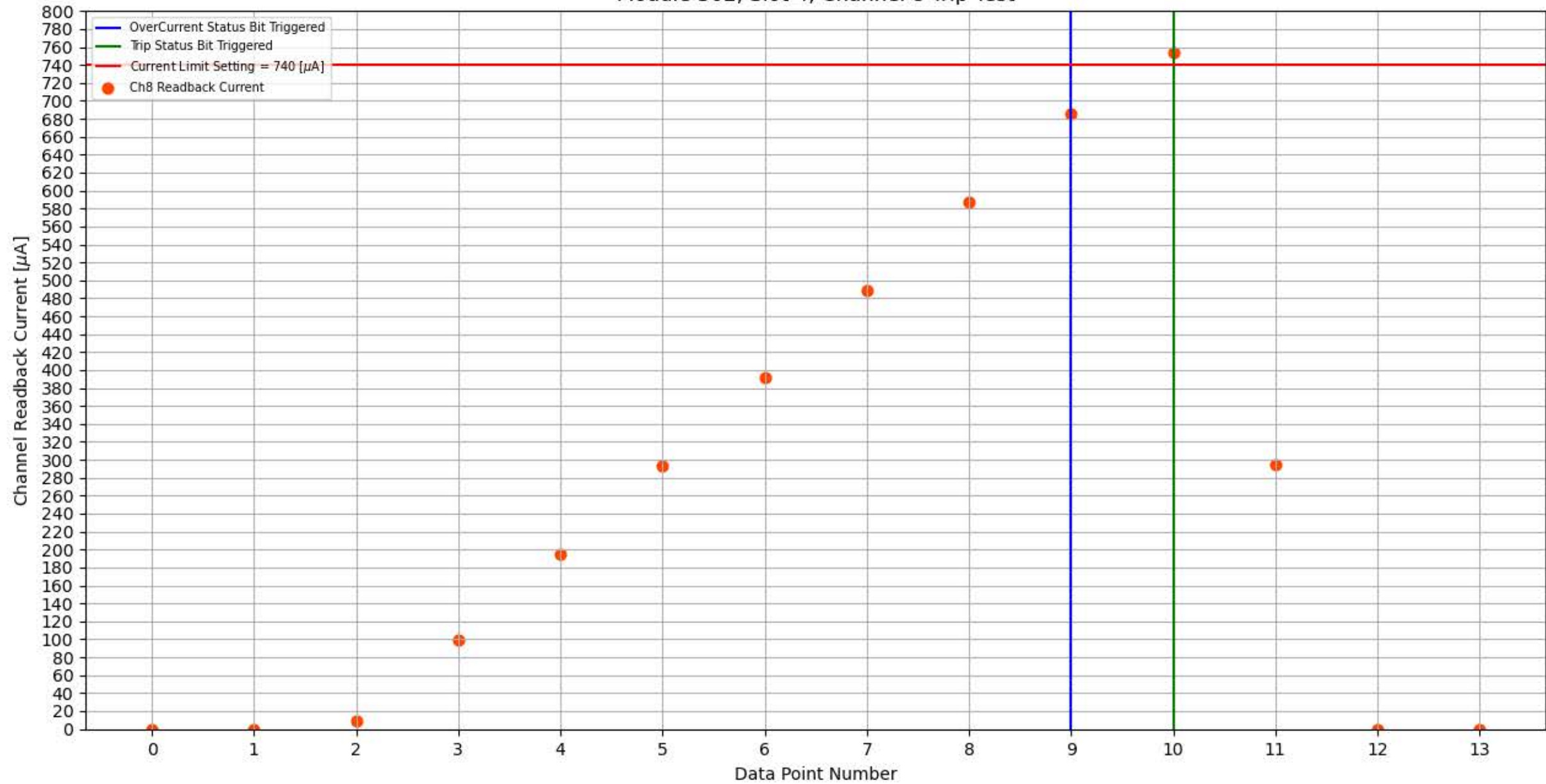
Module 302, Slot 4, Channel 8 Trip Test
