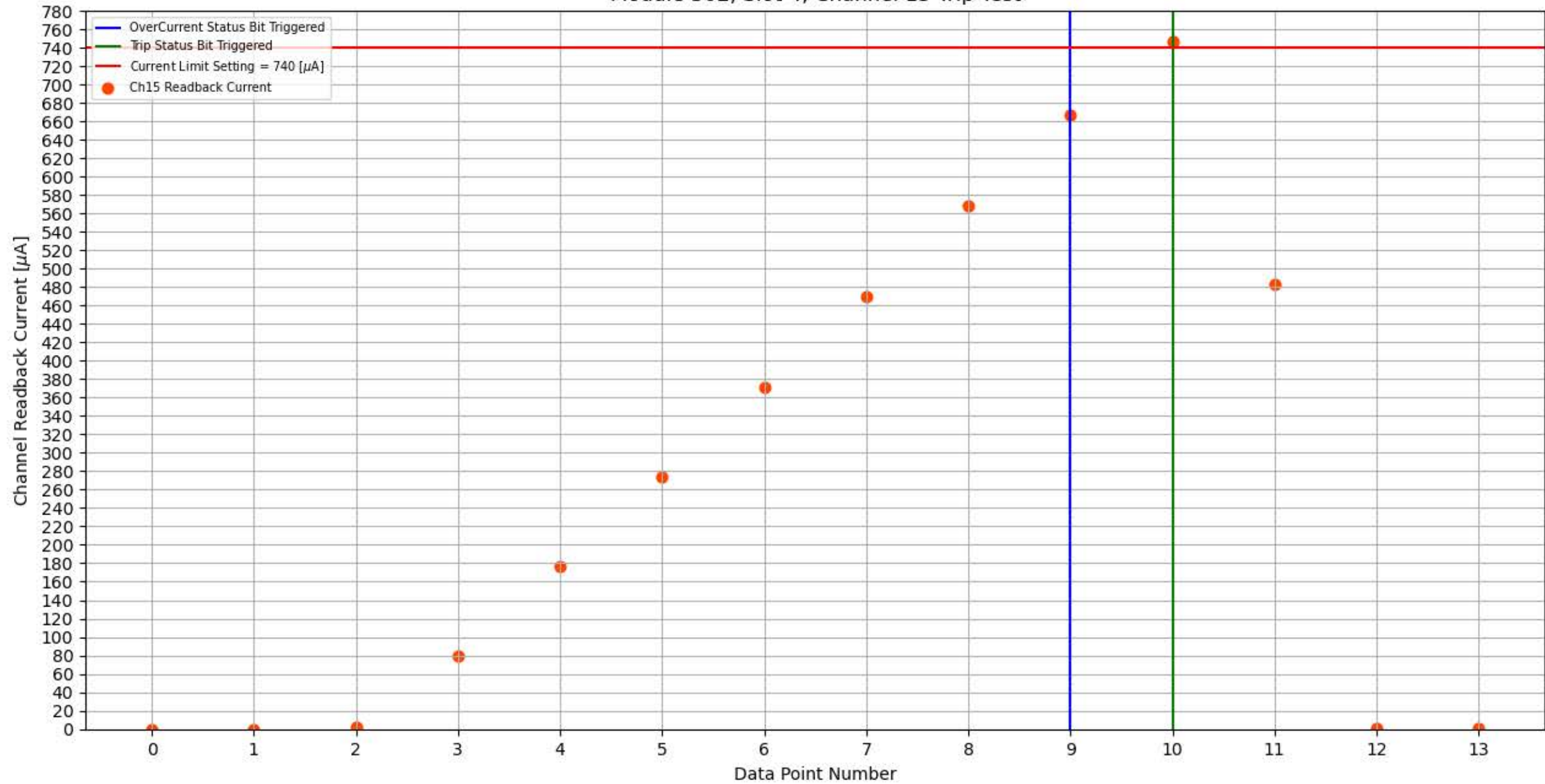
Module 302, Slot 4, Channel 15 Trip Test
