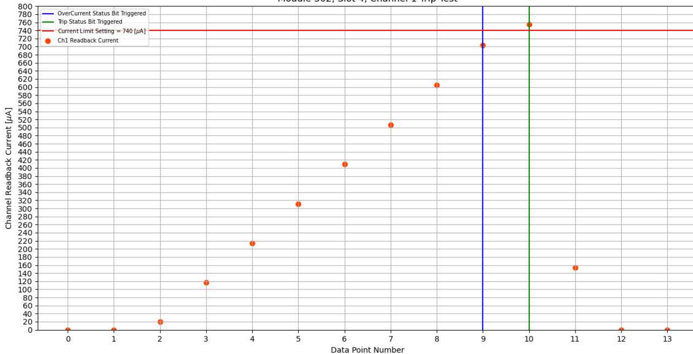
Module 302, Slot 4, Channel 1 Trip Test
