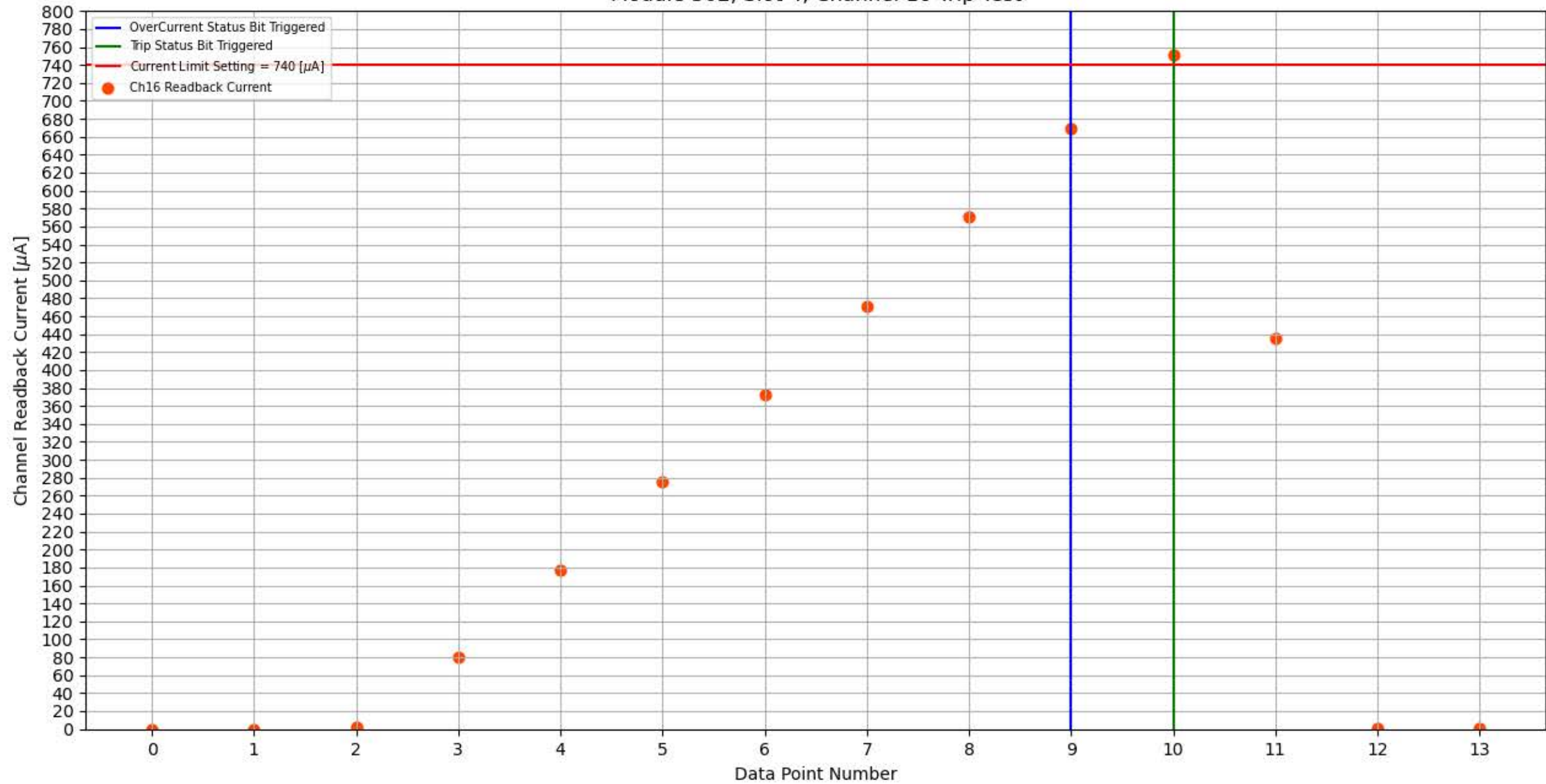
Module 302, Slot 4, Channel 16 Trip Test
