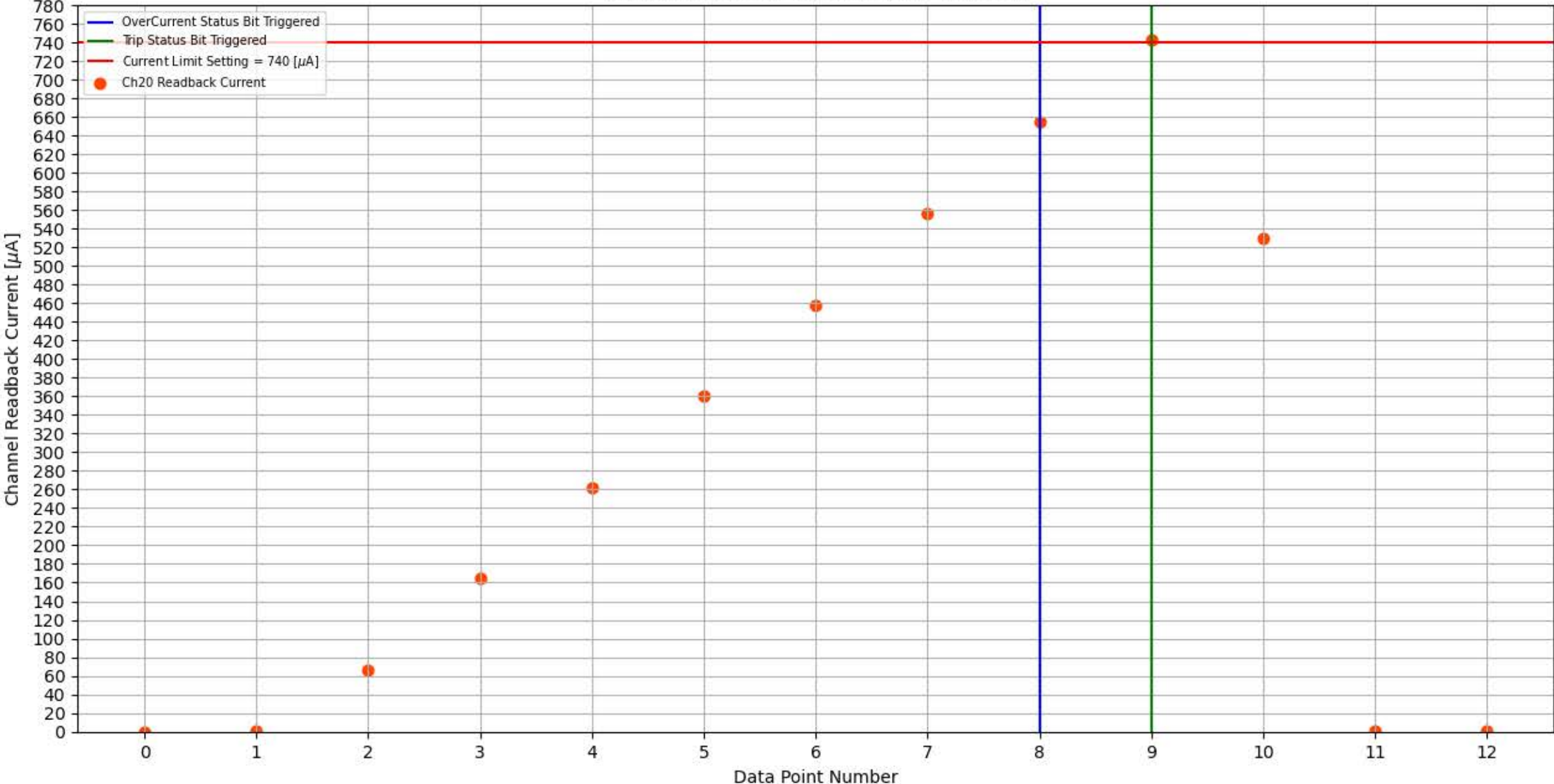
Module 302, Slot 4, Channel 20 Trip Test
