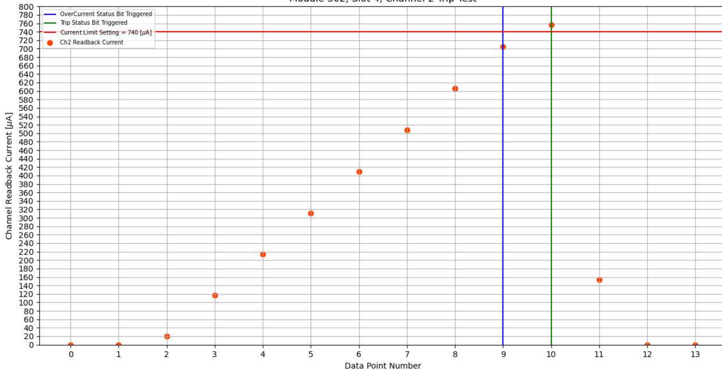
Module 302, Slot 4, Channel 2 Trip Test
