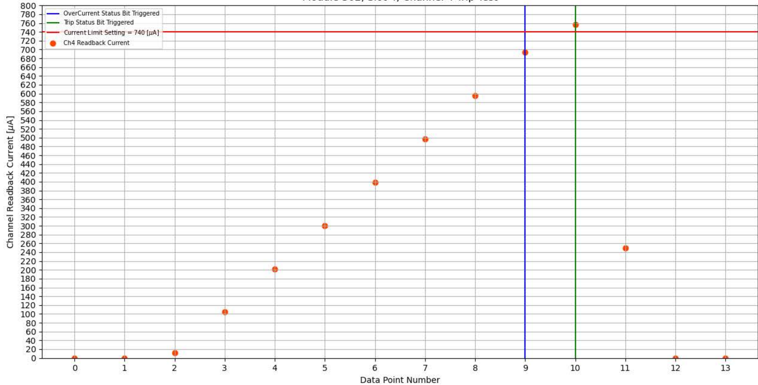
Module 302, Slot 4, Channel 4 Trip Test
