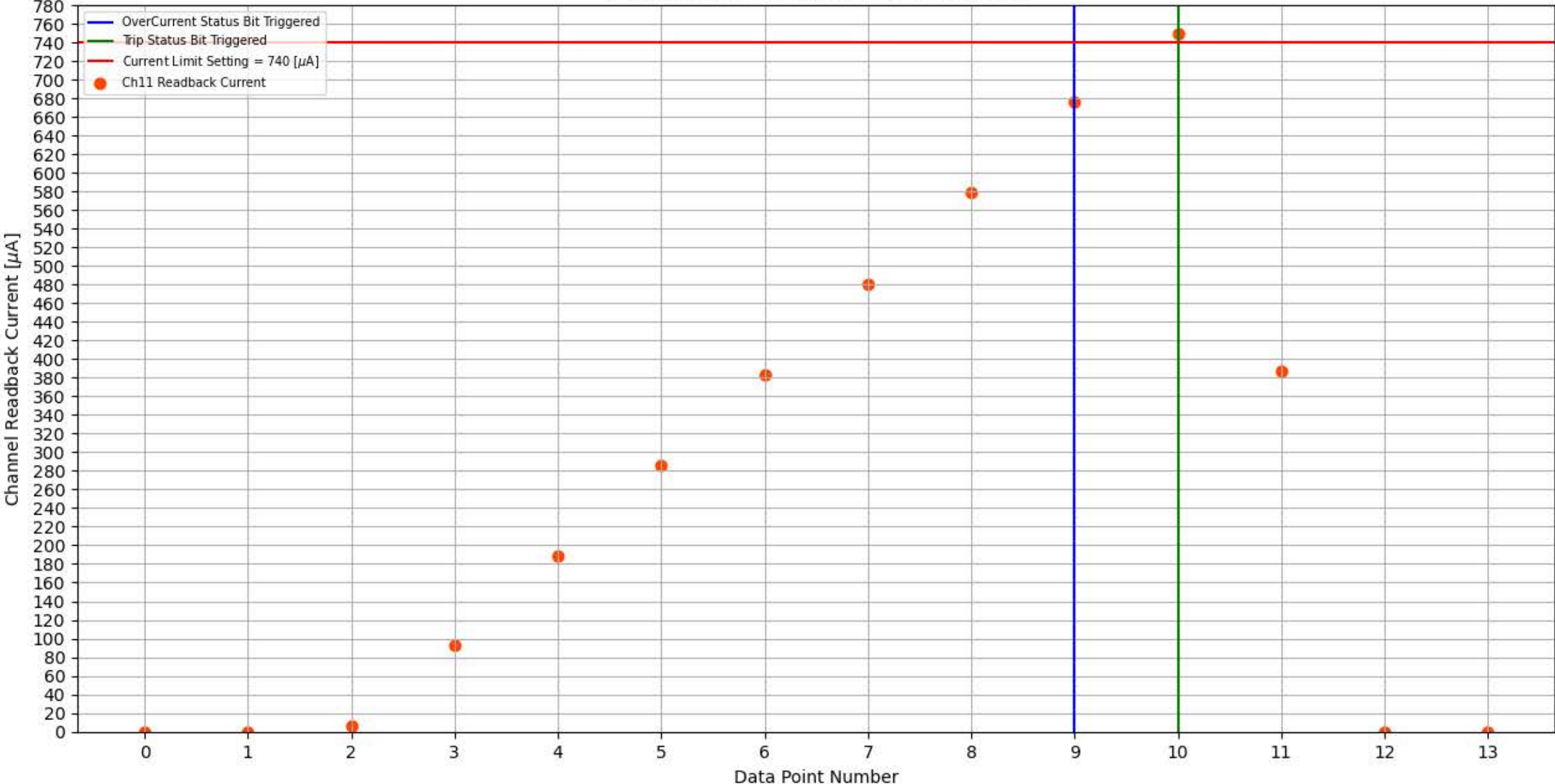
Module 302, Slot 4, Channel 11 Trip Test
